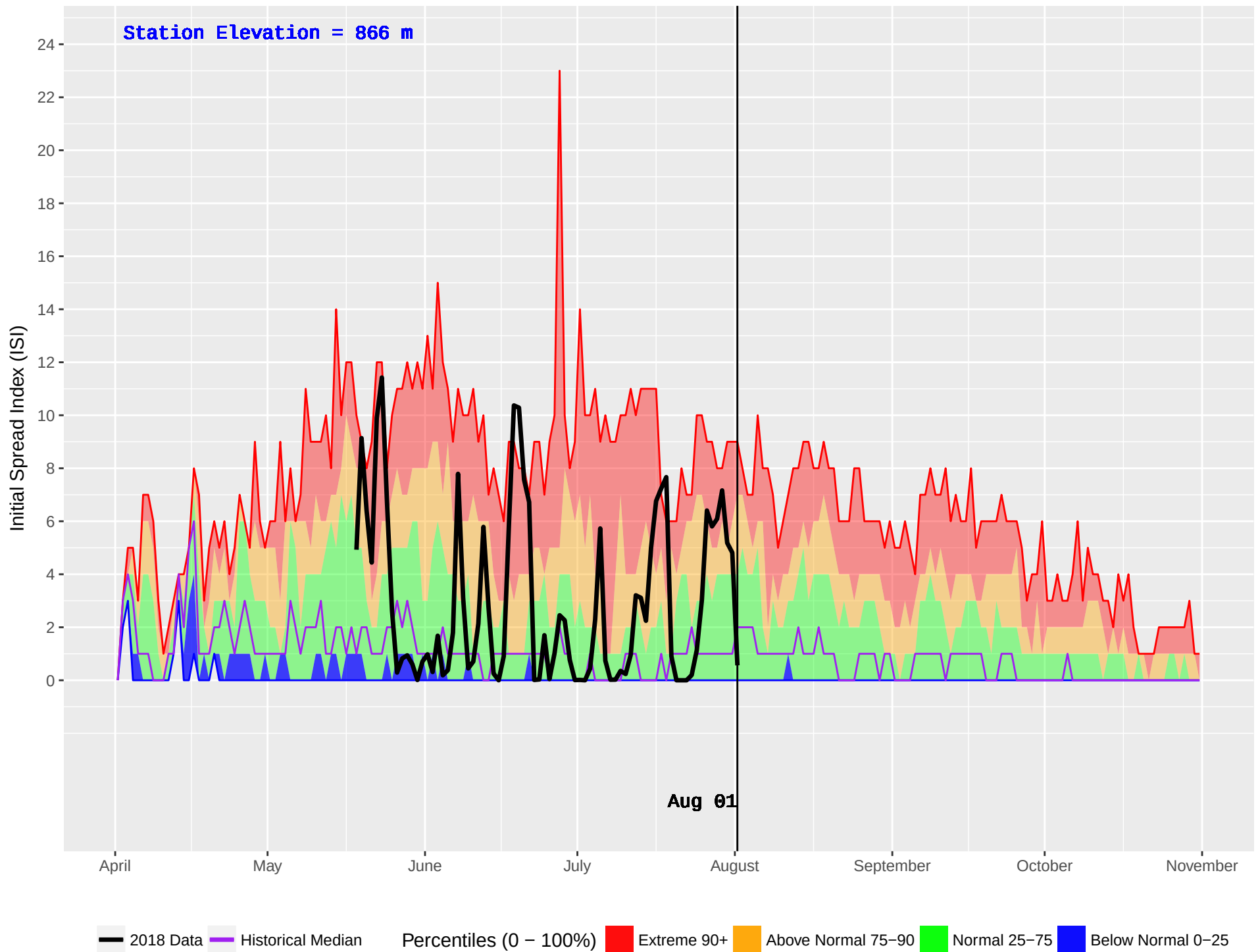
CATFISH (199) : Historical (1986–2016) and Current (2018) Daily Initial Spread Index (ISI)
