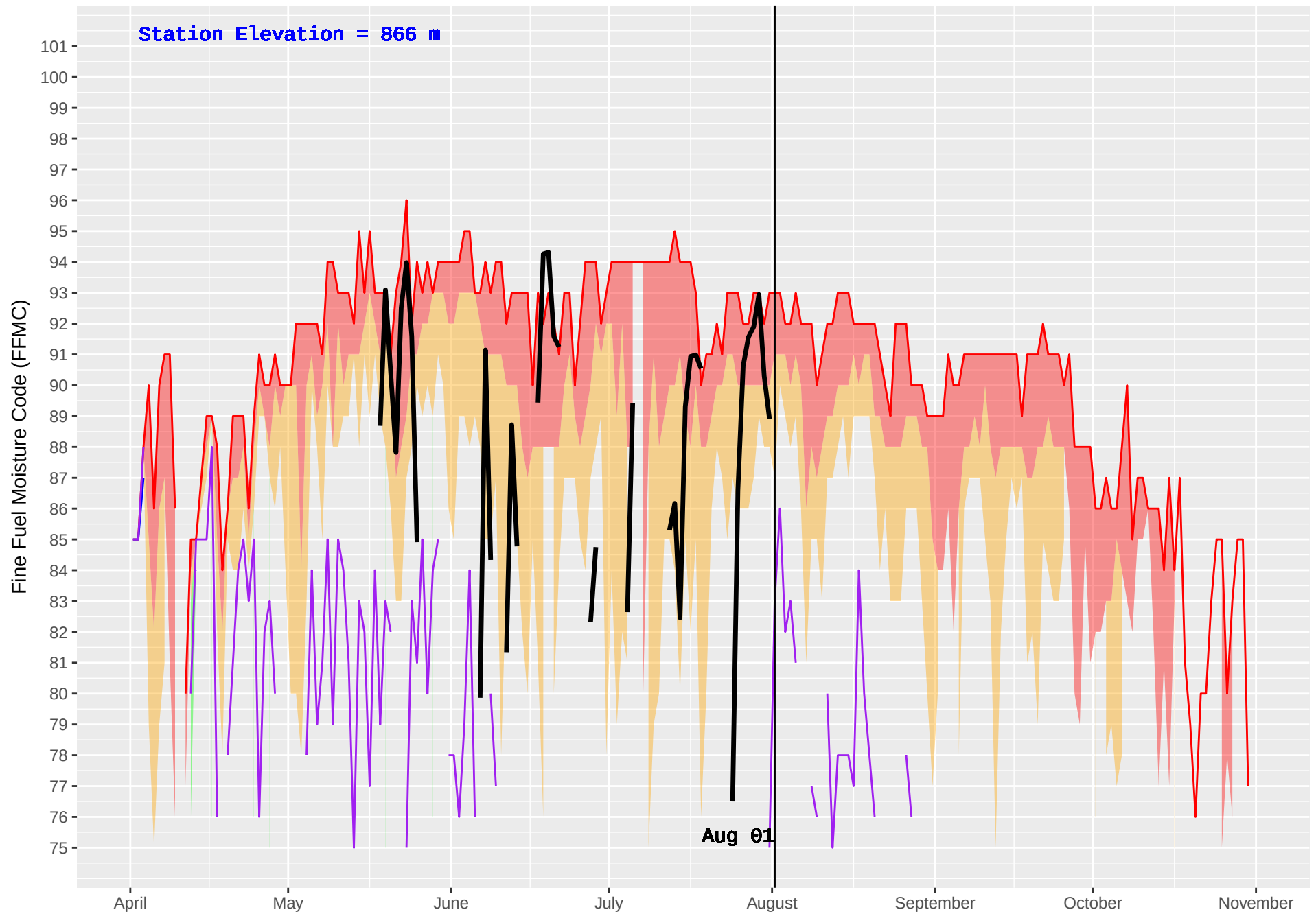
CATFISH (199) : Historical (1986–2016) and Current (2018) Daily Fine Fuel Moisture Code (FFMC)
