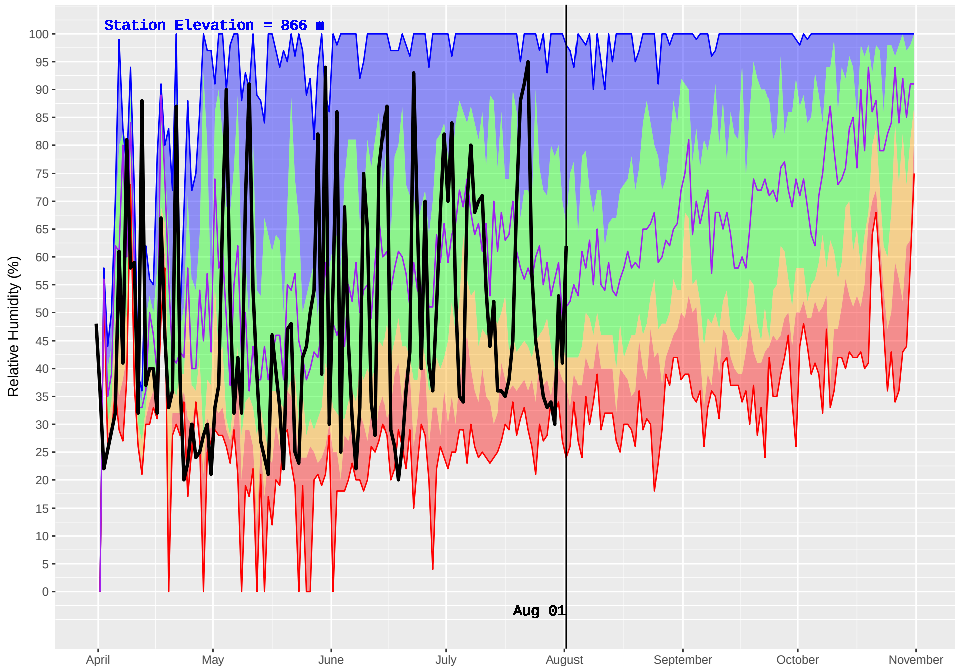
CATFISH (199) : Historical (1986–2016) and Current (2018) Daily Relative Humidity
